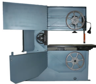
DT1340 with top and bottom doors open.
